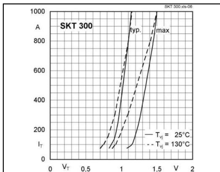
Fig. 6 On-state characteristics
